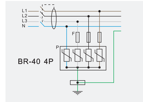
Common and differential mode protection
